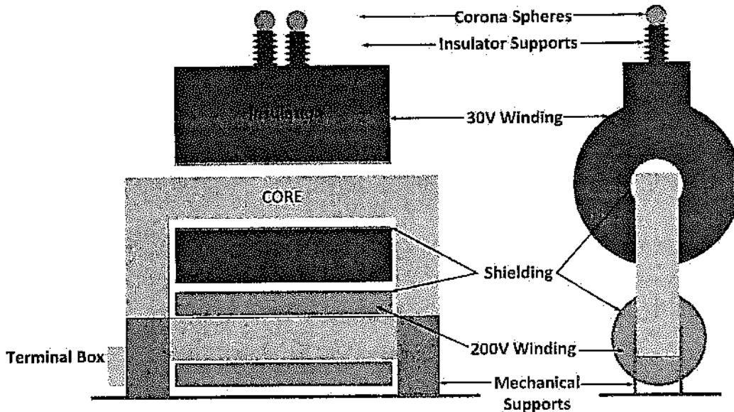
Figure 1 Suggested drawing
